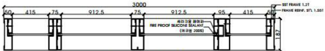
A-1 SECTION
